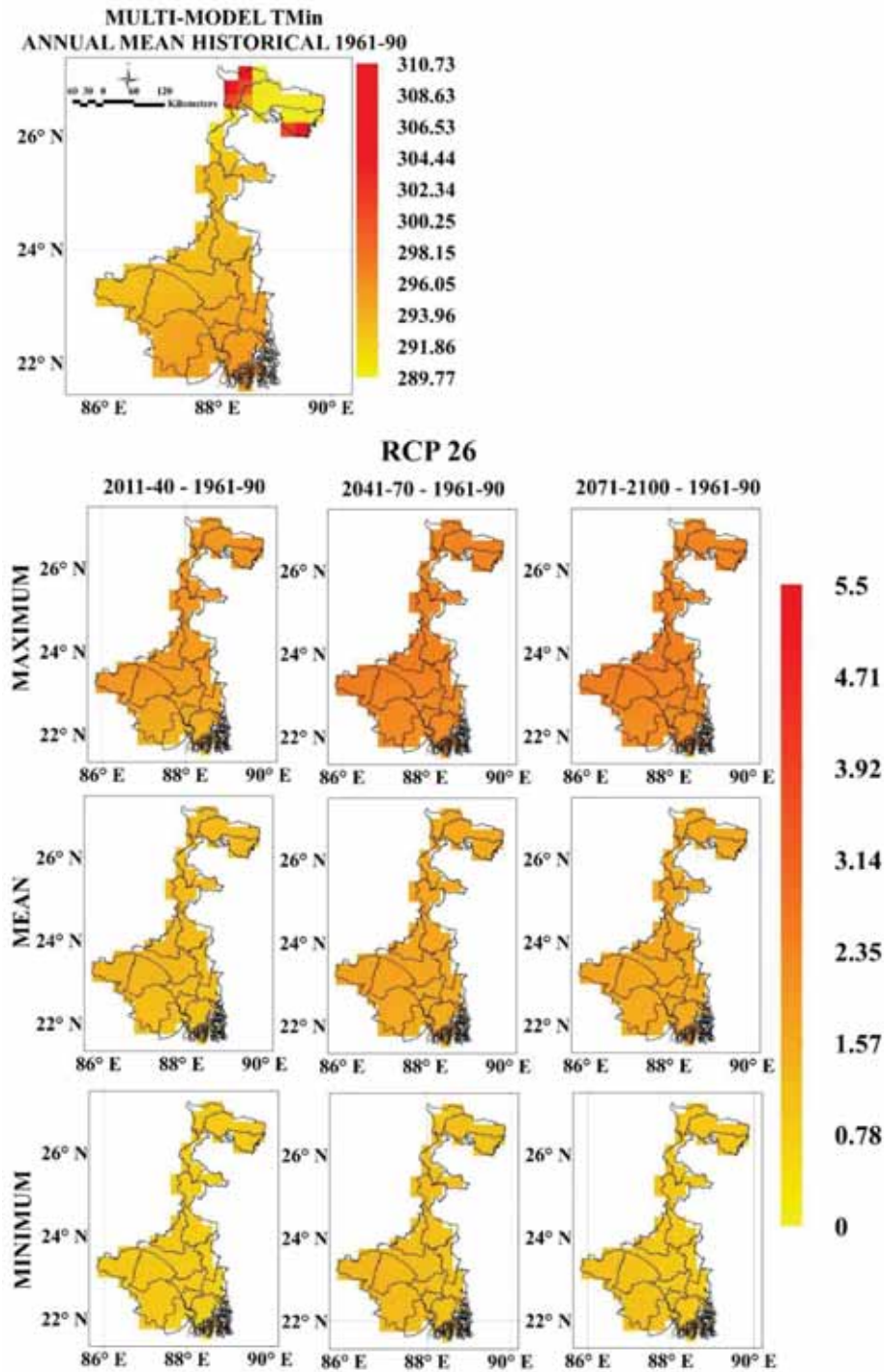
Figure 3.20: district level simulated (1961-1990) mean minimum temperature projections for the period 2011-2040, 2041-2070, and 2071-2100
