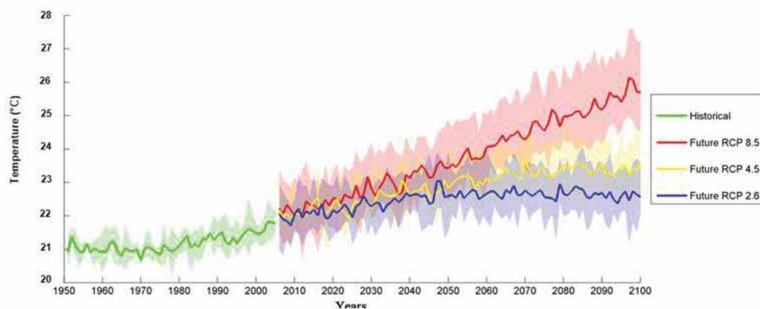
Figure 1.17: Simulated (1951-2010) and projected average annual minimum temperature trends in West Bengal
