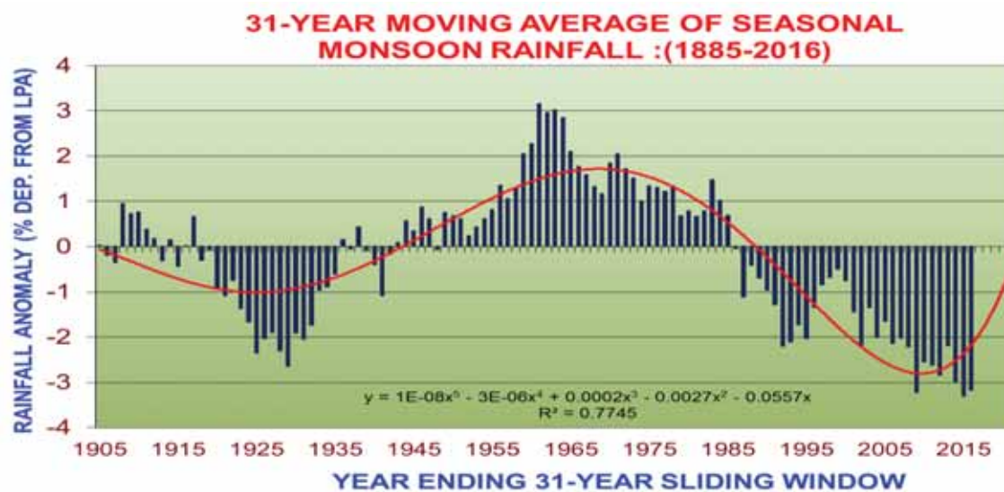
Figure 3.10: Availability of rainfall shows variability and availability of less rainfall during 1885-2015
