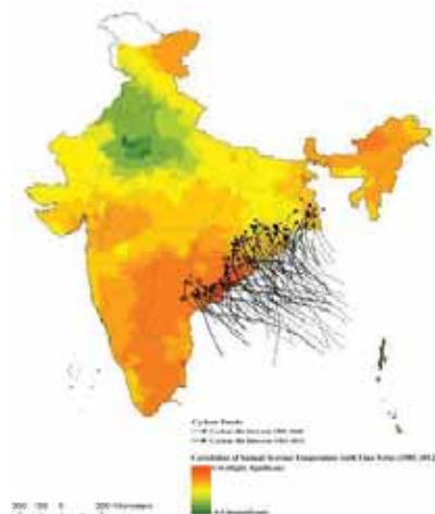
Figure 3.15: Cyclone Tracks Along The Bay Of Bengal Entering The East Coast Of India during 1901-2013 Source: Misra, 2014 9 .
