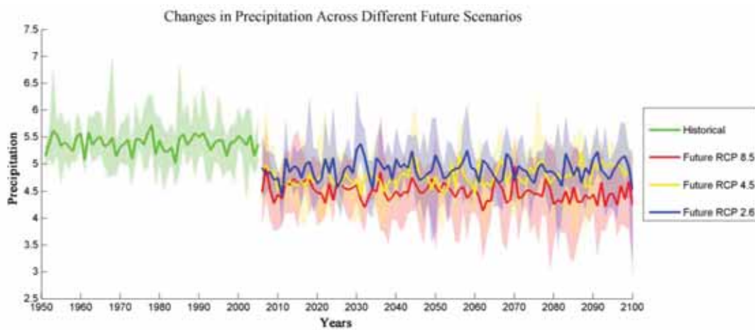
Figure 3.18: Simulated (1961-2010) and Projected (till 2100) changes annual precipitation intensity (mm/day)
