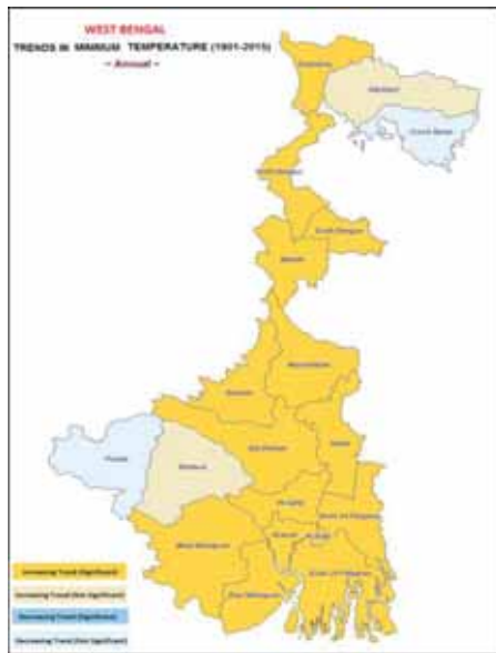
Figure 3.5 : Trends of Annual Minimum Temperature (1901-2015)
