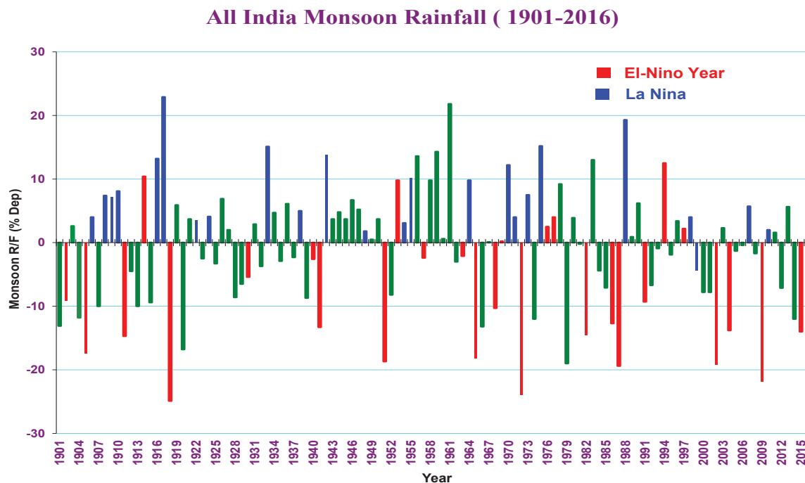
Figure 3.9 Indian Summer Monsoon is significantly influenced by El-Nino and La Nina Phenomena
