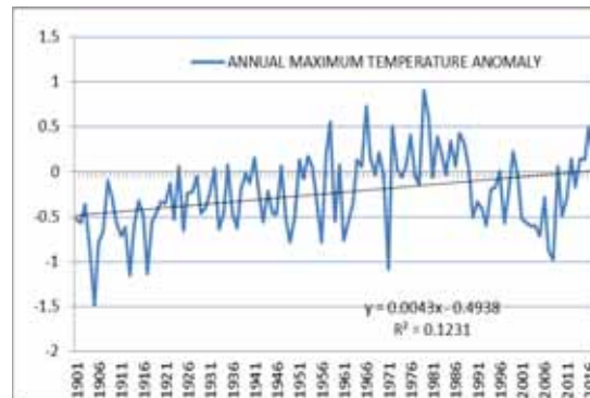
Figure 3.2: Annual maximum temperature anomaly for West Bengal for 116 yrs
