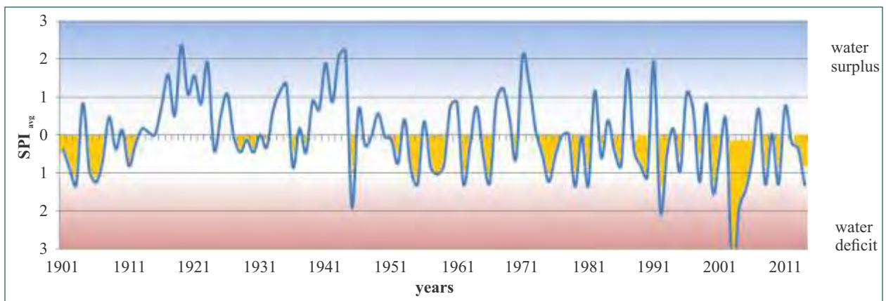
Fig. 5.a Temporal Evolution of 1-Month SPI for the Entire Kashipur & Chhatna Blocks
