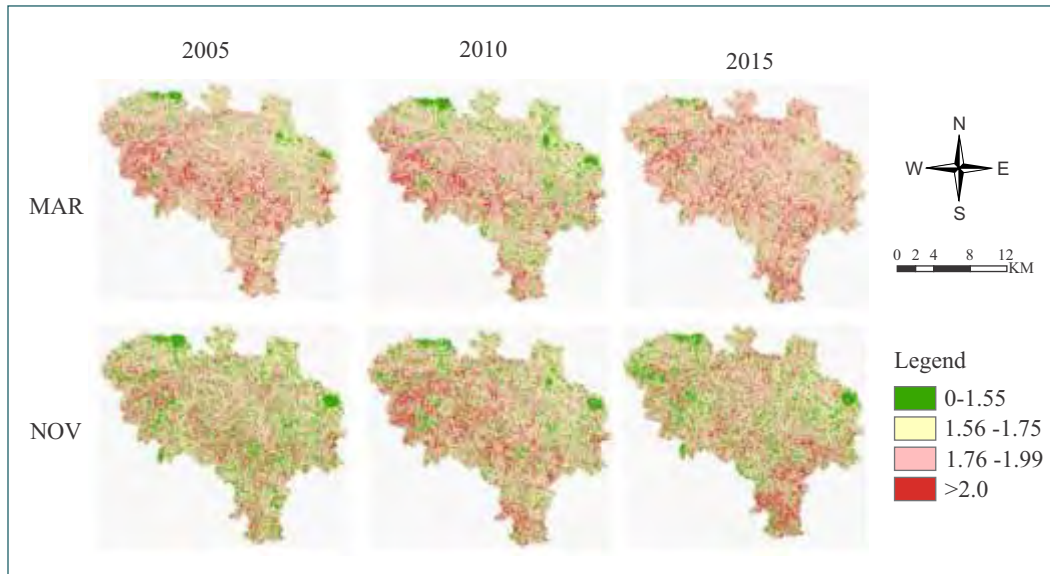
Fig. 5.d Moisture Stress Index of Kashipur & Chhatna Blocks in 2005, 2010 & 2015
