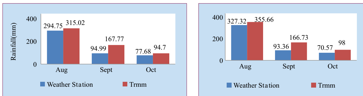
Fig 4.e Comparison Between Weather Station Data (Nutandi & Kroshjuri) and Satellite Data (TRMM)
