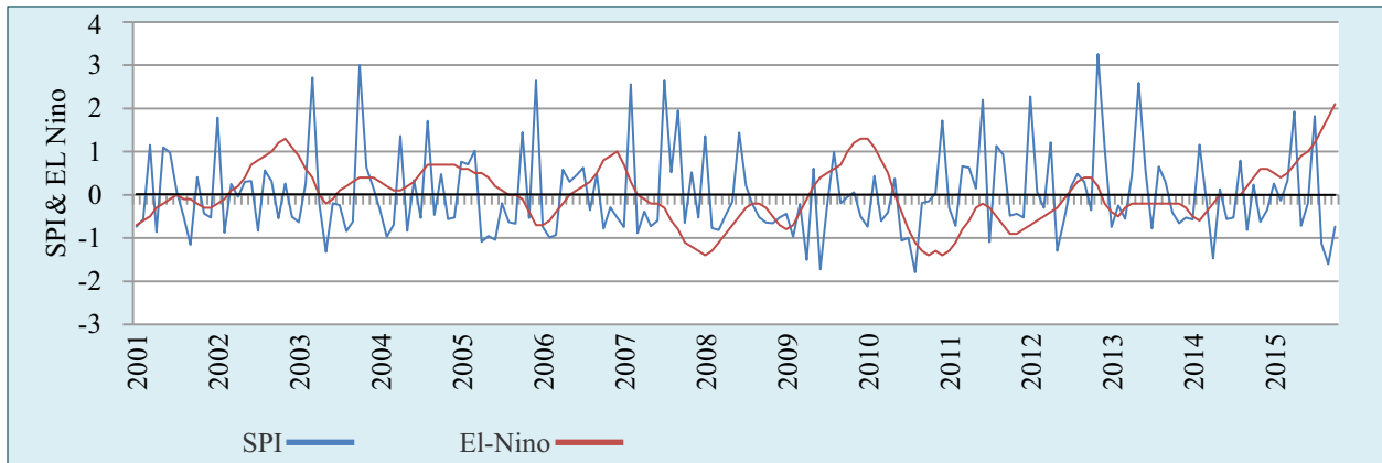
Fig 5.i Relation Between El-Nino & Drought Index
